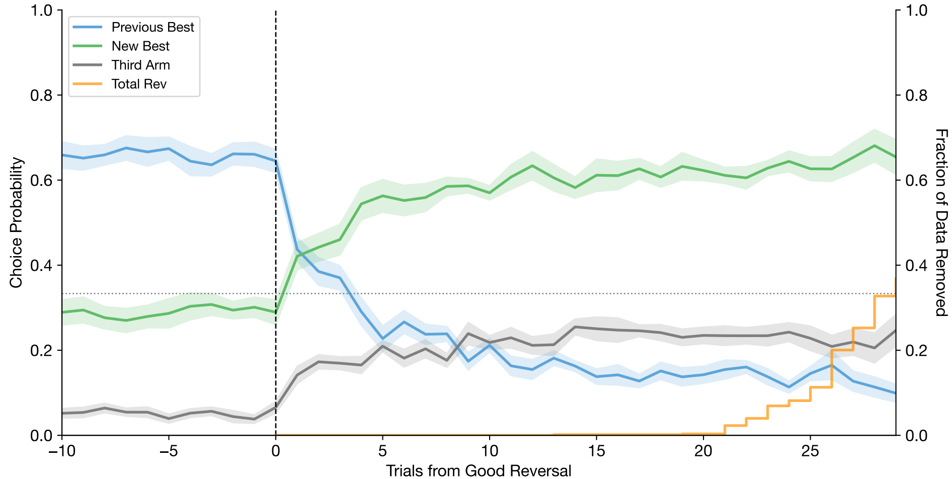
Reversal-Aligned Choices (mean \pm se across problems | n=6 subjects, n=548 reversals, n=14 problems)
